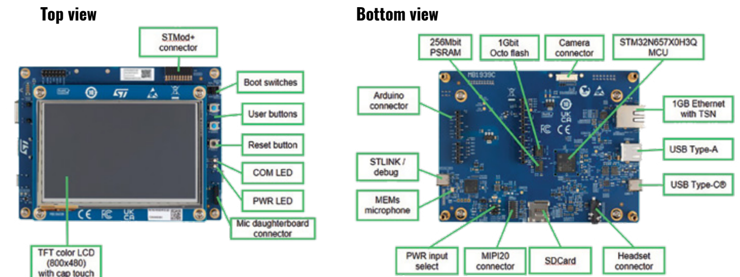
FIGURE 2: Picture showing the top and bottom views with different components
