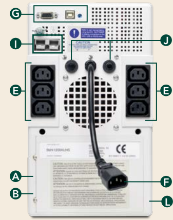
SMX1200XLHG UPS System (back)
