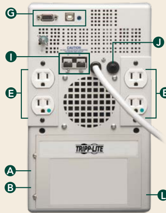
SMART1200XLHG UPS System (back)
