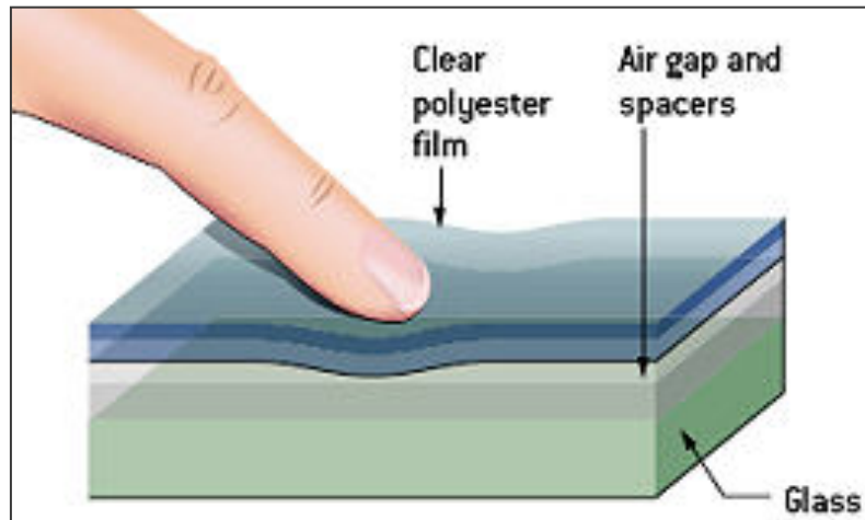
Resistive
