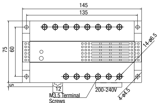
PS5R-E (100W)
