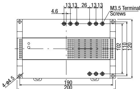
PS5R-G (240W)
