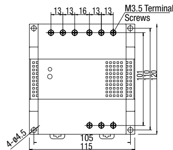
PS5R-TJ24
