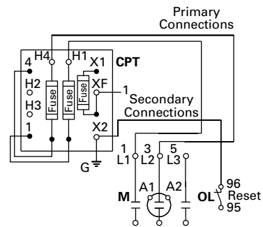
Figure 2 Fusible Control Transformer Remove Wire "C" (Figure 1) if Used and Connect as Shown Below. (All Other Starter Wires Remain as Shown in Figure 1)
