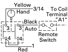
Figure C 3-Position Selector Switch
