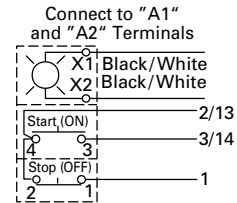
Figure F START/STOP with Pilot Light
