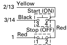
Figure B START/STOP Selector Switch
