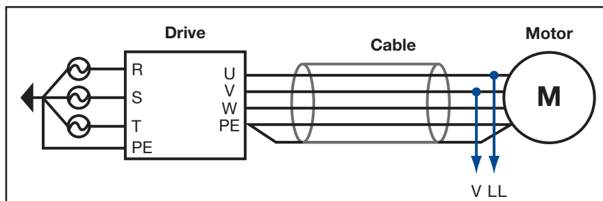
Figure 1. Schematic of a VFD setup.
