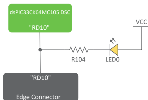
Figure 4-3. dsPIC33CK64MC105 Curiosity Nano LED0 Block Diagram
