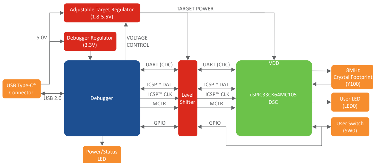
Figure 1-2. Block Diagram
