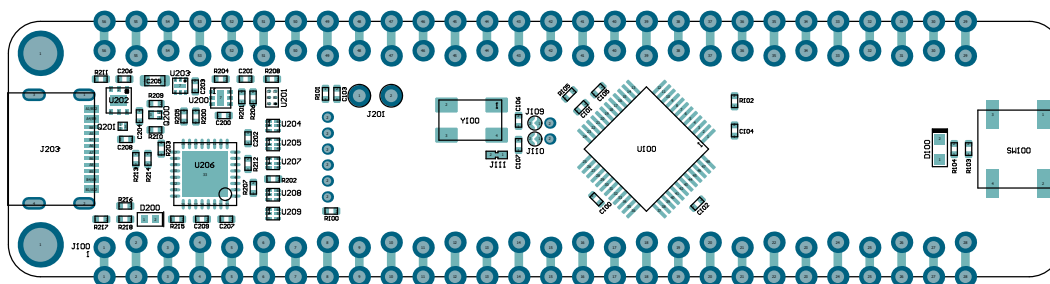
Figure 7-2. dsPIC33CK64MC105 Curiosity Nano Assembly Drawing Top
