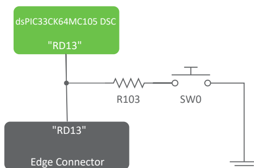
Figure 4-4. dsPIC33CK64MC105 Curiosity Nano SW0 Block Diagram
