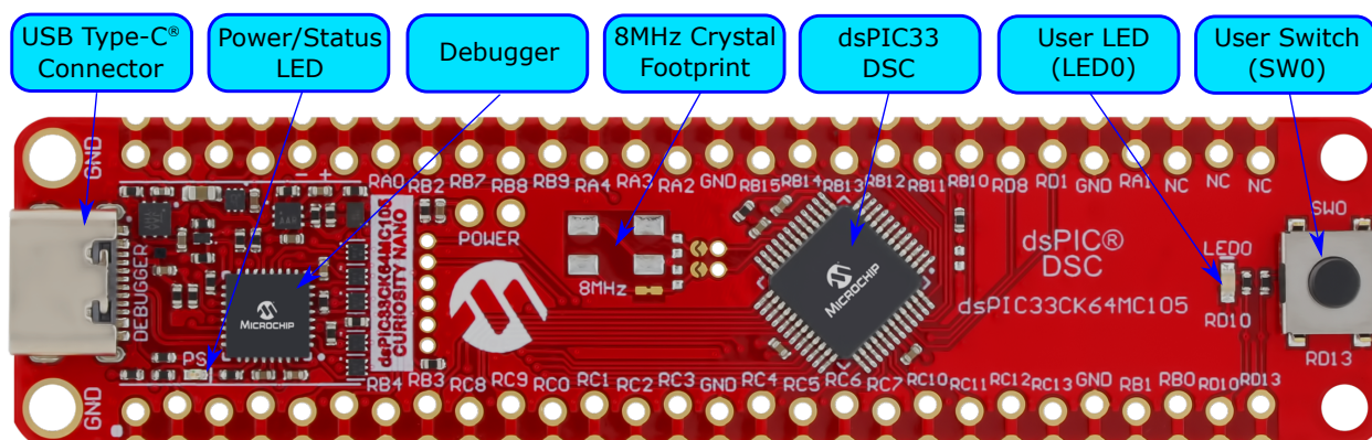
Figure 1-1. dsPIC33CK64MC105 Curiosity Nano Board Overview
