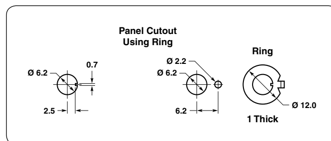
Recommended Hole Layout to Prevent Rotation
