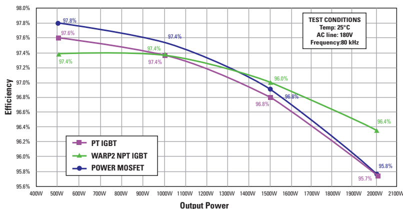
System Efficiency Comparison in a 2000W Power Supply
