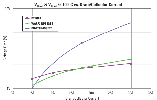
Voltage Drop vs. Current
