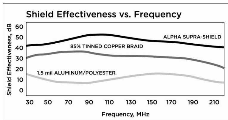
Figure 2. Foil-braid shielding yields the best shielding effectiveness
