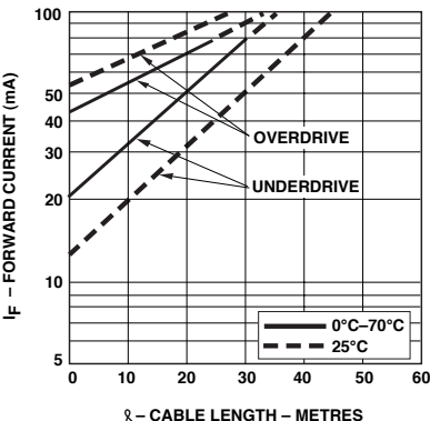
Figure 4. Guaranteed system performance with improved cable (HFBR-15X1Z/25X1Z)
